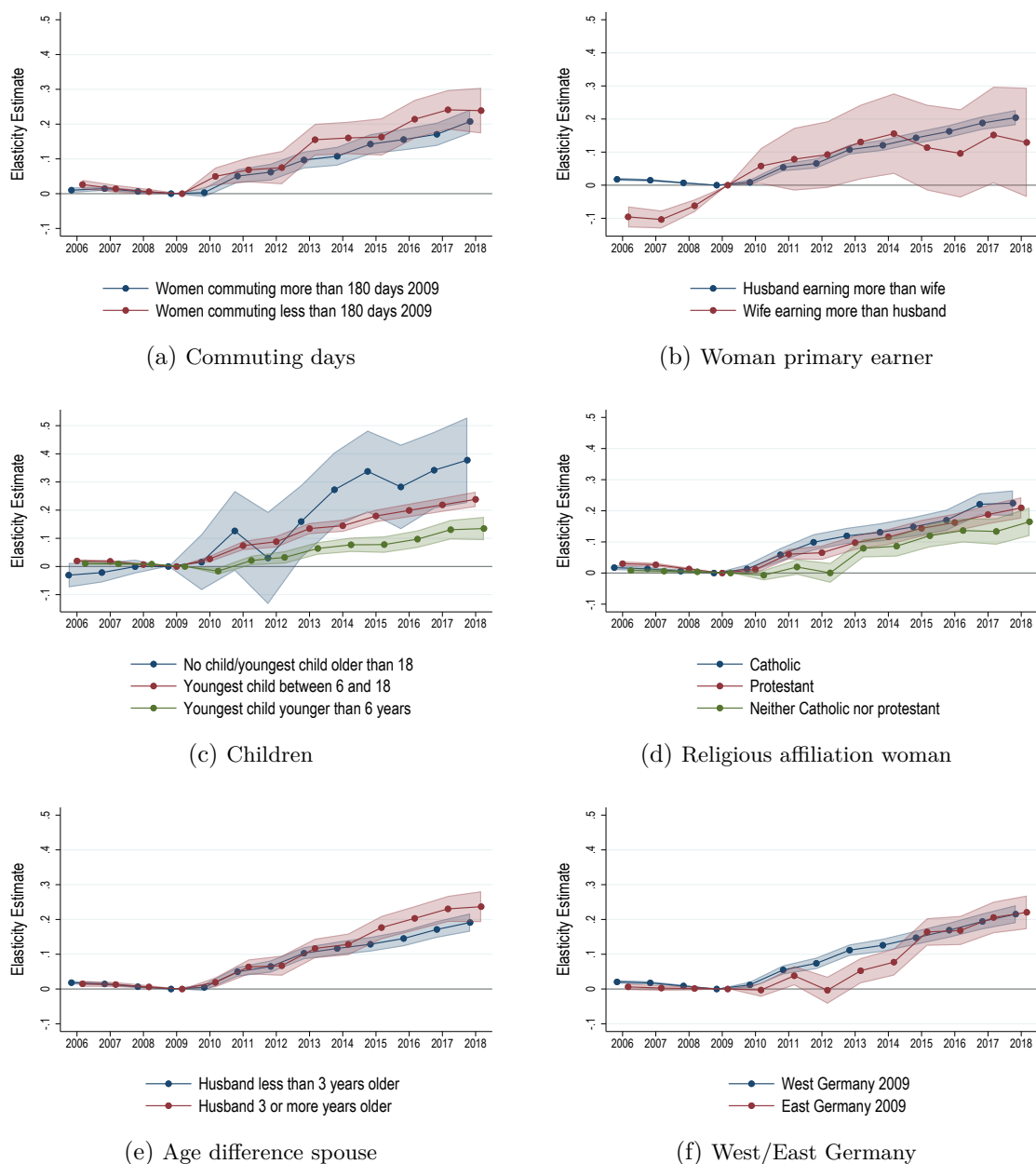
Figure 10: Effect Heterogeneity
